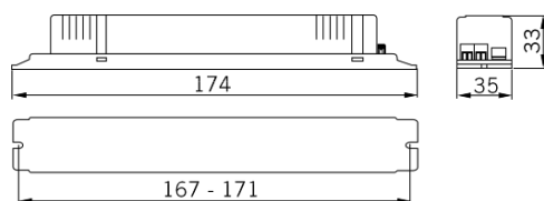
Driver
